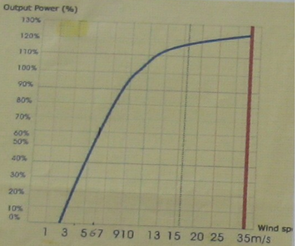
Power curve of 1kW~5kW VAWT
